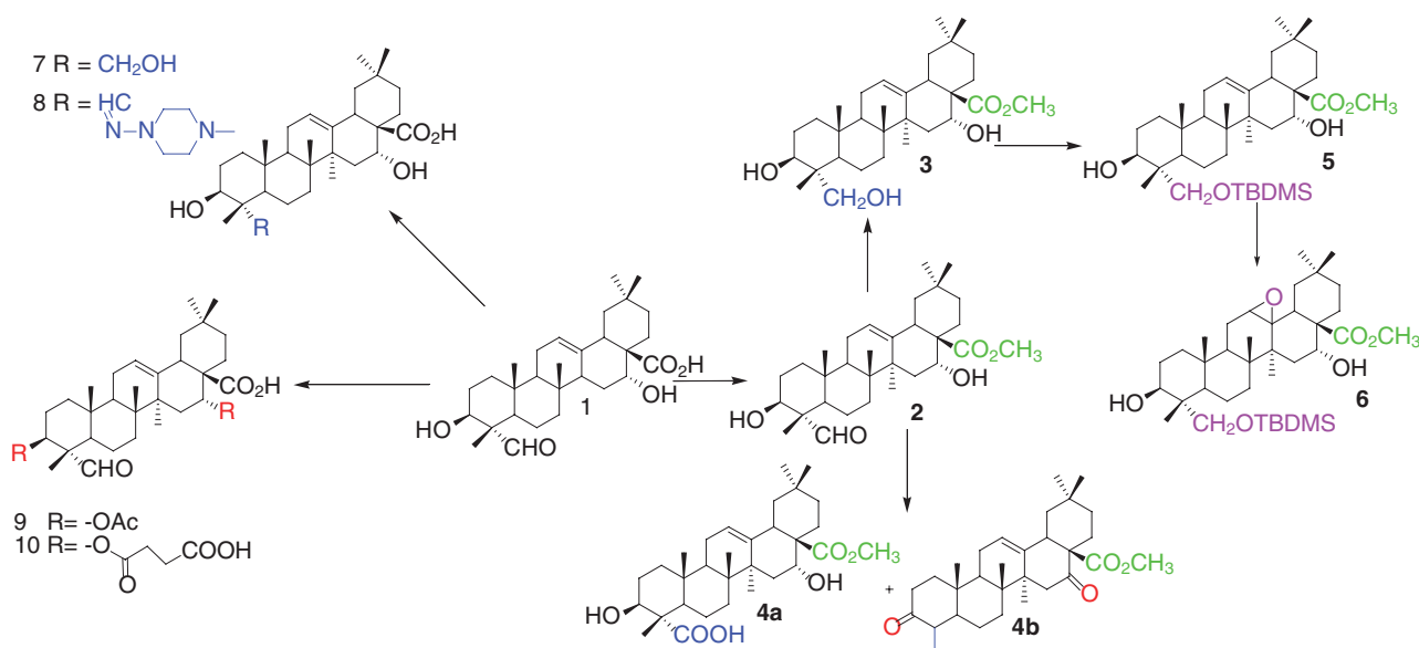
Figure 1 Structure of quillaic acid ( 1 ), the major aglycone of quillaja saponin, and derivatives.
